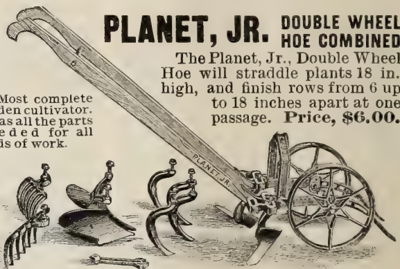
PLANET, JR., DOUBLE WHEEL HOE COMBINED.
